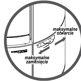
Picture 6 Adjustment of air inflow in DEFRO HOME ORION stove: upper controller controls the flow of secondary air, bottom controller controls the primary air.
