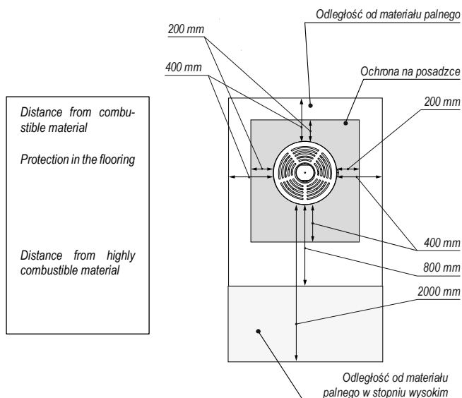
Figure 3.3 Minimum safe distances during setting of dry stove.
