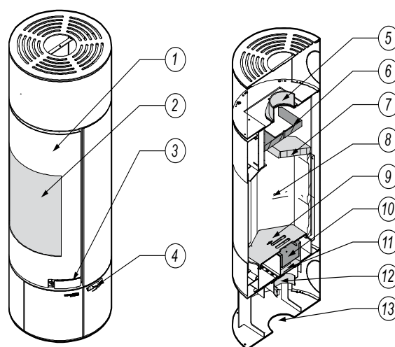
Picture 1. DEFRO HOME ORION dry stove design.
