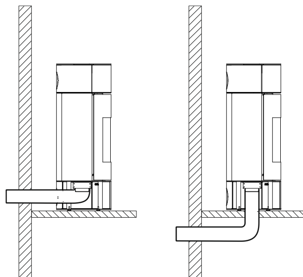
Picture 4.4 Connection of the DEFRO HOME ORION stove to the external air inlet.
